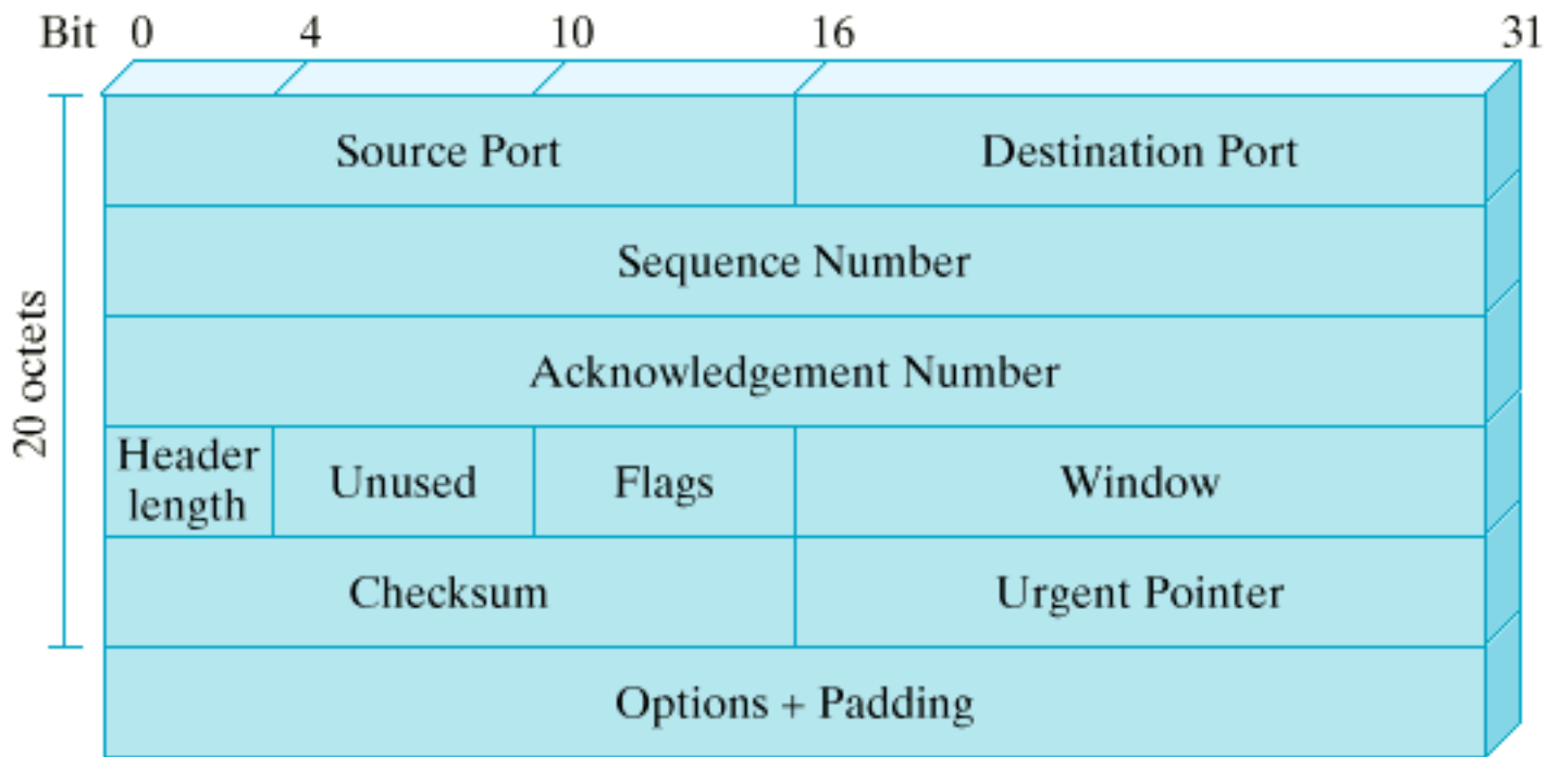
(a) TCP Header
