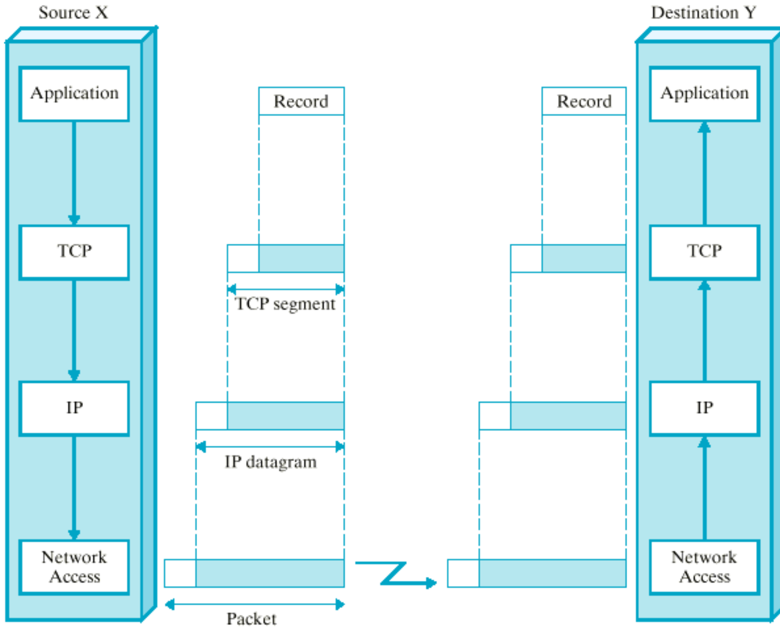
Figure 13.5 Operation of TCP/IP
