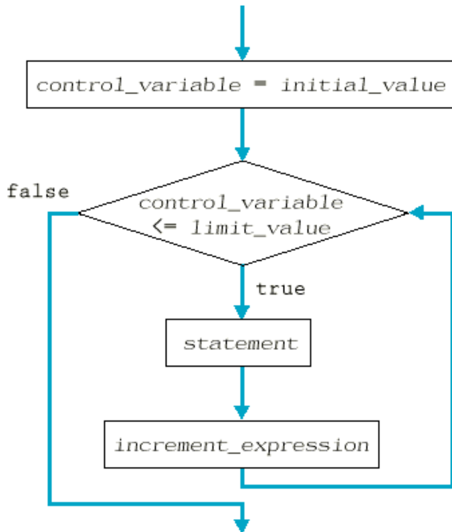
Ascending Form of a for Loop
